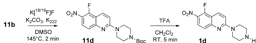
Scheme 7. Preparation of 5-fluoro-6-nitroquipazine ( 1d ) as an analytical reference.
