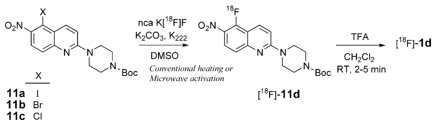
Scheme 6. Radiosynthesis of 5- [\text{18F}] fluoro-6-nitroquipazine ( [\text{18F}]\text{-1d} ).
