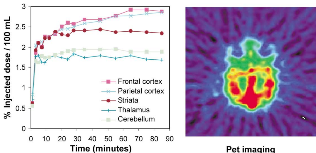
Figure 3. PET imaging of 5-[ ^{18}\text{F} ]fluoro-6-nitroquipazine ([ ^{18}\text{F} ]- 1d ) in Macaca fascicularis . Monkey was i.v. injected with 2.6 mCi (96.2 MBq) of 5-[ ^{18}\text{F} ]fluoro-6-nitroquipazine ([ ^{18}\text{F} ]- 1d ) and imaged for 90 min. The scanning protocol consisted of 16 images (5×2 min, 5×4 min, 6×10 min). During PET acquisition, arterial blood samples were withdrawn from a femoral artery at designated times. For data analysis, regions of interest (ROI) were placed on the frontal and parietal cortex, the cerebellum, the striata and the thalamus. The correct anatomical localization of the ROIs were checked on the MRI images. The radioactivity measured in each ROI was corrected for attenuation and fluorine decay and expressed as percent injected dose per 100 mL of tissue (% I.D./100 mL).
