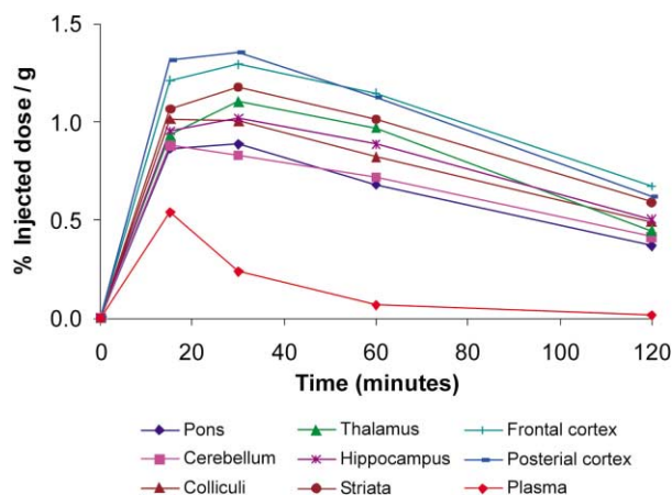
Figure 2. Time course of 5-[ ^{18}\text{F} ]fluoro-6-nitroquipazine ([ ^{18}\text{F} ]- 1d ) in Sprague-Dawley rats for 0–120 min. Twelve adult male Sprague-Dawley rats (weight 250–300 g) were i.v. injected in the tail vein with 5-[ ^{18}\text{F} ]fluoro-6-nitroquipazine ([ ^{18}\text{F} ]- 1d , 22–26 \mu\text{Ci} or 0.81–0.96 MBq). Animals were sacrificed 15, 30, 60 and 120 min after injection of the radiotracer ( n=3 per time point). The brain was quickly removed and dissected. Samples of cerebellum, pons, colliculi, thalamus, hippocampus, striata, frontal cortex, posterial cortex and plasma were obtained for each animal, weighed and their radioactivity measured in a \gamma -counter (Cobra Quantum, Packard). Tissue concentration were expressed as percent injected dose per gram tissue (% I.D./g).
